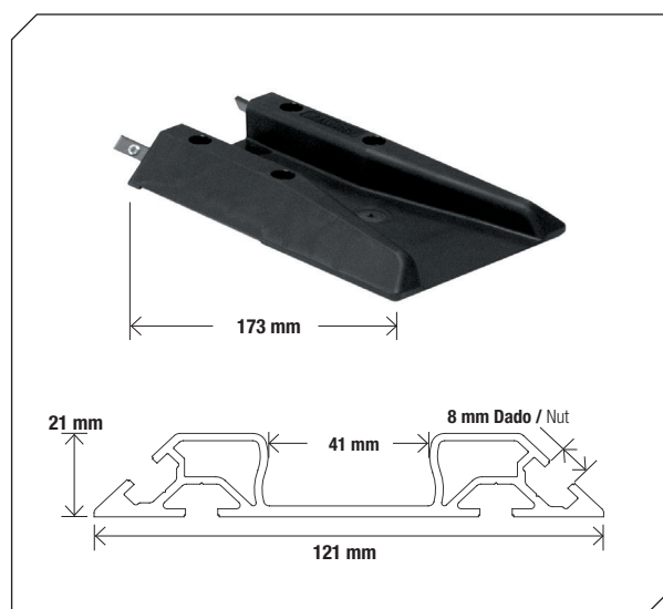
Terminale Fifo Monorail 40 mm / Terminal Fifo Monorail 40 mm
