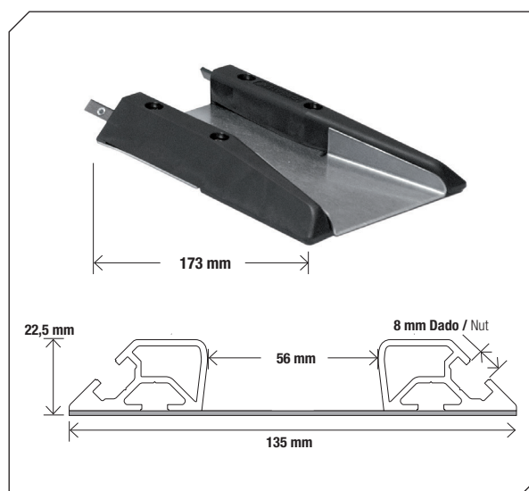
Terminale Fifo Monorail 55 mm / Terminal Fifo Monorail 55 mm
